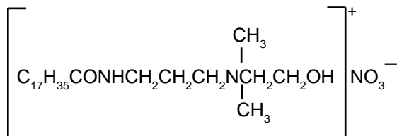
Stearamidopropyldimethyl-2-hydroxyethylammonium nitrate
