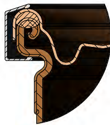
DETAIL B SCALE 1 : 1 TOP CHIME DETAIL
