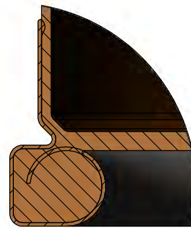
DETAIL C SCALE 1 : 1 BOTTOM CHIME DETAIL
