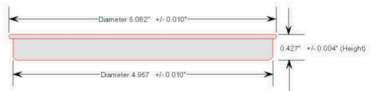
PLUG SIDE VIEW
