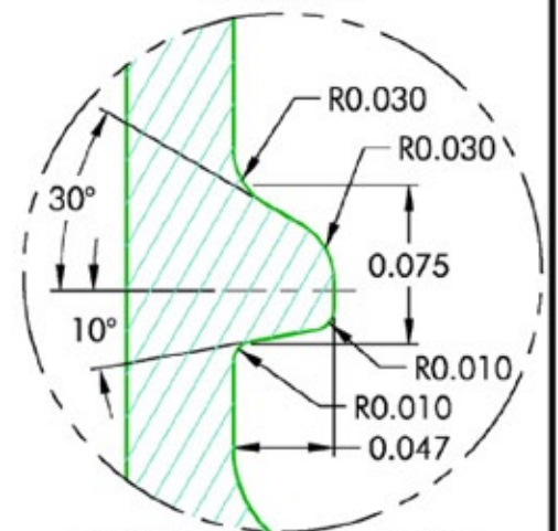
PLASTIC THREAD DETAIL SCALE 10 : 1
