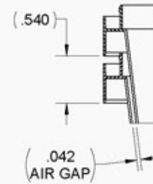
NESTING VIEW
