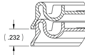
NESTING VIEW
