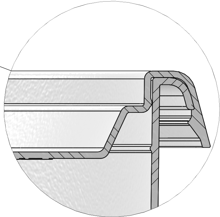
DETAIL B SCALE 5 : 1
