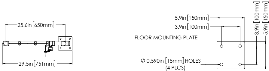
MOUNTING PLATE VIEW (MOUNTING HARDWARE NOT INCLUDED)
