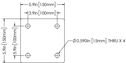
MOUNTING PLATE VIEW (MOUNTING HARDWARE NOT INCLUDED)
