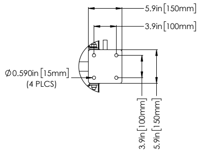
MOUNTING PLATE VIEW (MOUNTING HARDWARE NOT INCLUDED)
