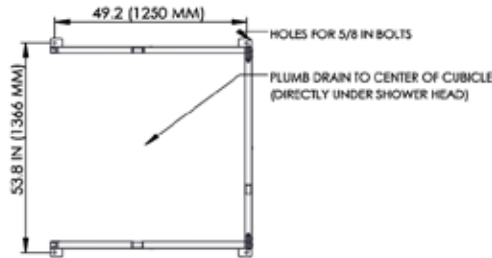
PLAN VIEW DETAILING FOOTPRINT
