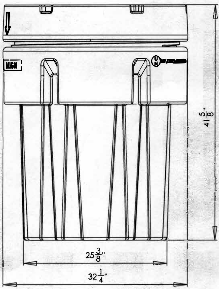
SIDE VIEW
