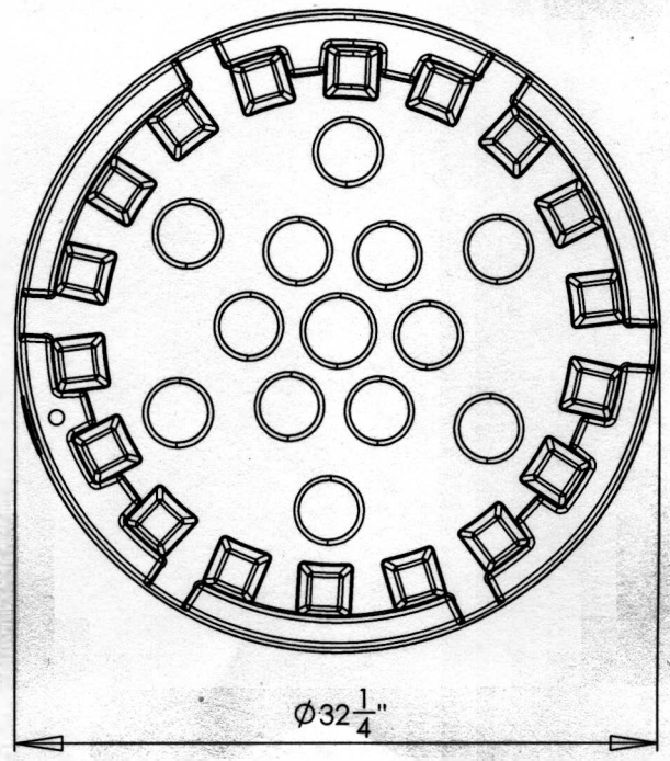
PLAN VIEW
