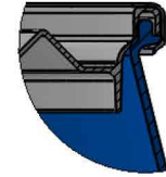
DETAIL D SCALE 1 : 2 TOP CHIME DETAIL WITH COVER AND RING
