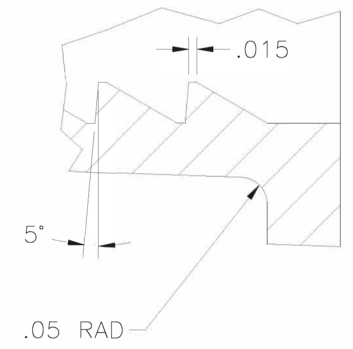
THREAD DETAIL SHOWN 4X SIZE
