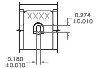
WIRE EAR OPENING SCALE 2:1
