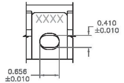
PLASTIC EAR OPENING SCALE 2:1
