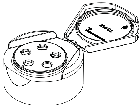
.200" SIFT HOLE (5X) REFERENCE PART WEIGHT: 6.13g
