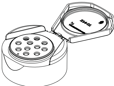
.125" SIFT HOLE (11X) REFERENCE PART WEIGHT: 6.14g
