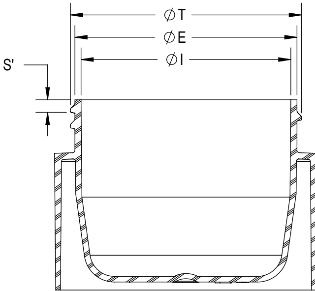
SECTION G-G
