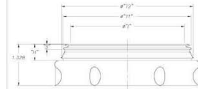
110 MM XLV CAP SNAP
