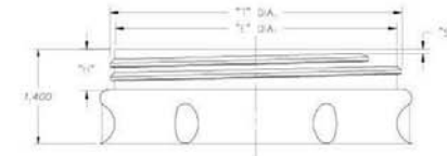
110 MM SP-400 M-STYLE 1.5 TURNS OF THREAD
