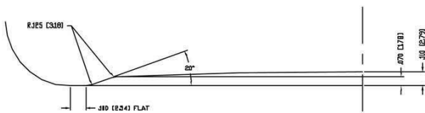
PUSH UP DETAIL SCALE: 3-1
