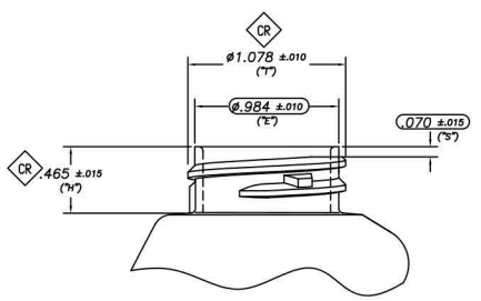
28-P-1530 NECK FINISH MODIFIED BUTTRESS THREAD.
